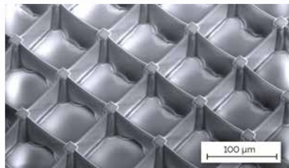
Cage structures made of circa 50 \mu m thick SU-8. The structures are used in biological applications to trap and grow cells.
