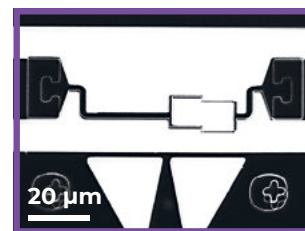
An optical image of the transmon's tunable SQUID, with its flux bias above it.
