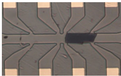
2D Materials: optical micrograph of a \text{Bi}_2\text{Sr}_2\text{CaCu}_2\text{O}_{8-x} exfoliated onto a thin film of \text{Ga}_{1-x}\text{Mn}_x\text{As} . The film was then etched into a double hall-bar structure around the flake.
