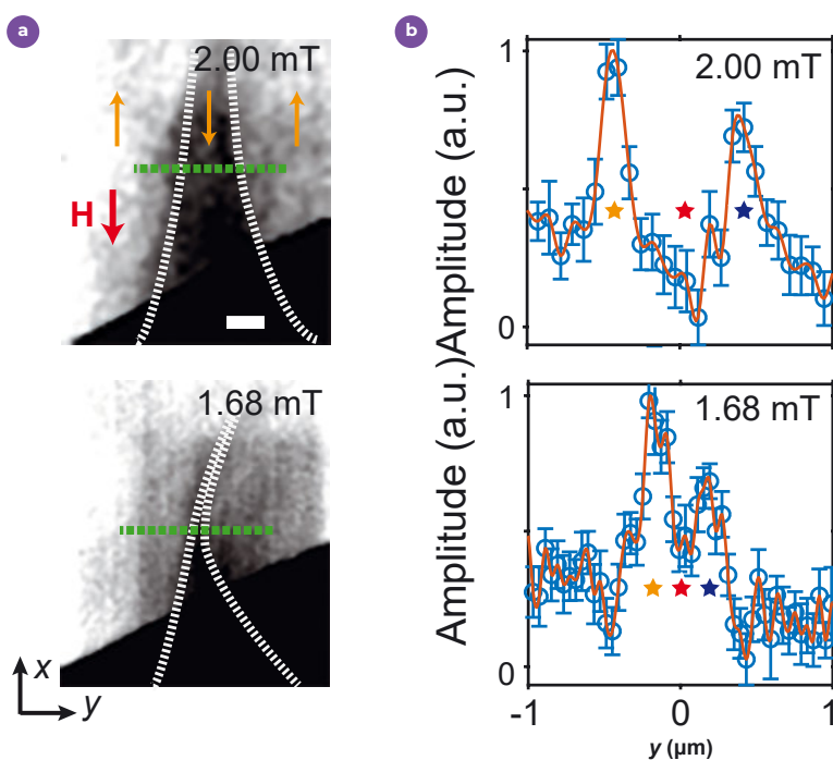
Fig. 5. Static STXM image of a circuit composed by two domain walls sharing an apex. By varying the external field the two domain walls are displaced from far (top) to close (bottom). Scale bar 500 nm; Corresponding spin-wave intensity along the green profiles of panel a. 5
