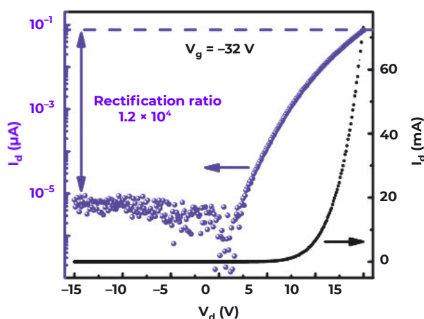
The output curve of the lateral p-n junction in logarithmic (left axis) and linear scale (right axis), obtained at the optimal back gating of -32 V.
