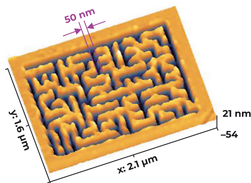
AFM image of a "labyrinth" patterned by thermal nanocutting. Image courtesy Dr Xia Liu, EPFL.
