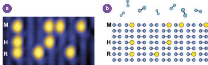
STM image (a) and a schematic (b) of the 24-bit memory array after the interdimer sites have reacted with hydrogen molecules, thereby rewriting the stored information. The remaining hydrogen gas in the chamber does not react with the isolated DBs in the array and can be used in further rewriting operations.
