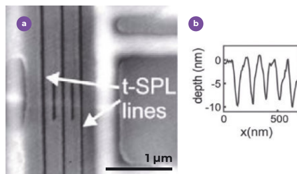
Figure 2: NanoFrazor image of the top gates patterned in the PPA resist; (b): line scan along the nanowire.
