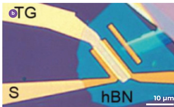
a : Optical image of a single-layer MoS 2 flake with Hall bar FETs patterned on it; b : Top-gated MoS 2 FET with h-BN as a gate dielectric. Both devices show exceptional performance due to improved source-drain charge injection. 3
