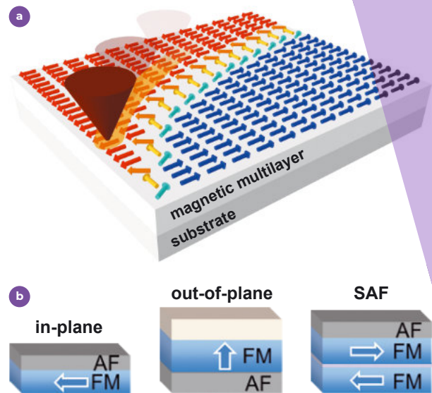
Fig. 2, : Sketch of tam-SPL; : Different exchange bias systems where tam-SPL has been demonstrated.
