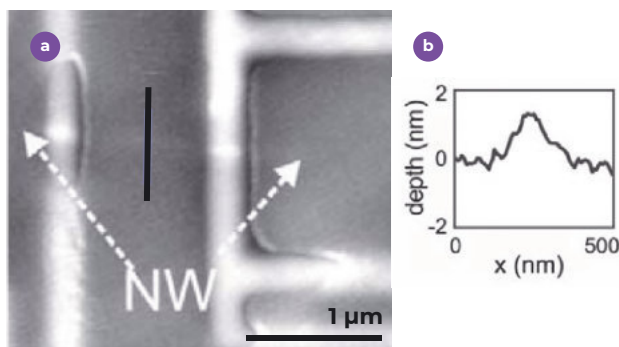
Figure 1: NanoFrazor image of the 30 nm-thick InAs NW with Au contacts under 200 nm of the resist; (b): line scan along the line on the left.
