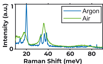
Air-Sensitive Materials: Raman spectra measured on \alpha\text{RuCl}_3 showing the difference exfoliation in the inert atmosphere makes. Raman measurements were taken inside the glovebox.
