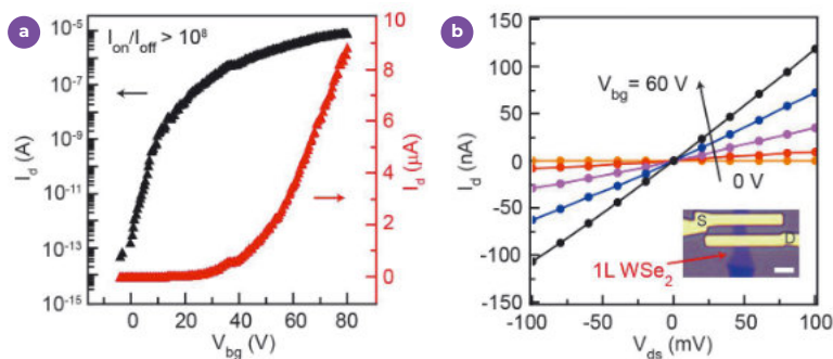
Characteristics of FETs fabricated via t-SPL on exfoliated 1L WSe 2 flakes. a : Transfer curves acquired at room temperature with V_{ds} = 2 V for back-gated FETs fabricated on monolayer exfoliated WSe 2 , featuring an I_{on}/I_{off} > 10^8 . The transfer curve is shown both in the linear scale (red triangles) and log scale (black triangles). b : Corresponding room temperature output curves at different gate voltages ( V_{bg} ). In the inset, optical image of the t-SPL device. Scale bar: 2.5 \mu m
