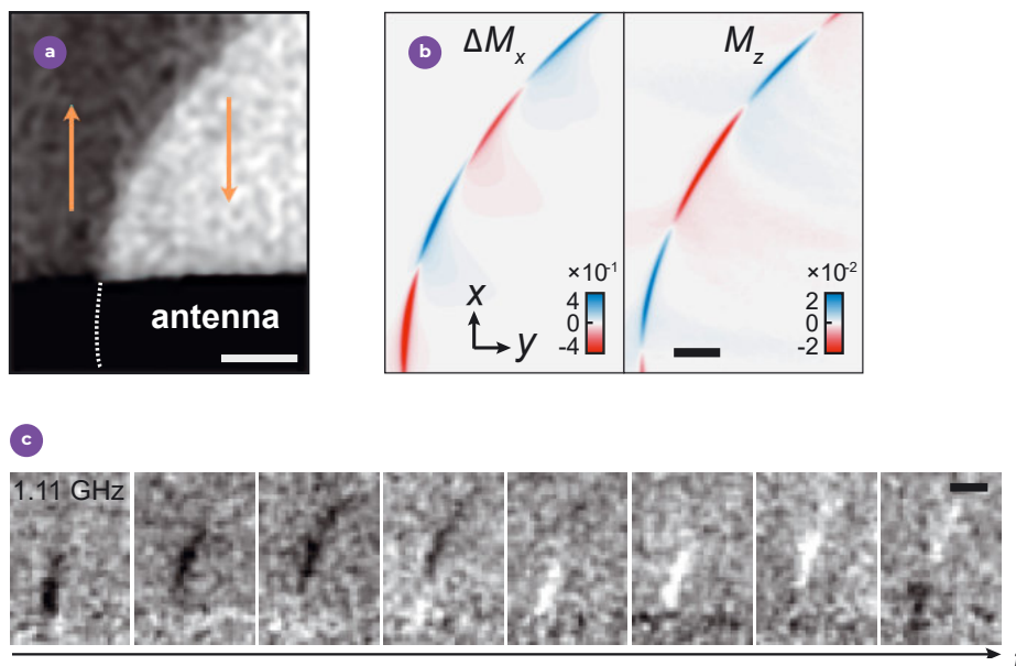
Fig. 4. (a): Static STXM image of a curved wall; (b): Micromagnetic simulation of spin waves propagating and confined within the curved wall, (c): Sequence of STXM images showing the confinement, propagation and steering of spin waves within the domain wall. Scale bars: 500 nm. 5
