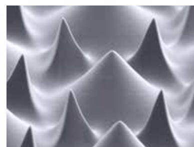
Diffuser: Resist AZ 4562, structure size < 5 µm
