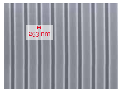
Minimum feature size: 300 nm - or even less. The image shows the result of a high-resolution test exposure with a nominal linewidth of 250 nm!
