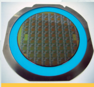
Mounted Wafer
